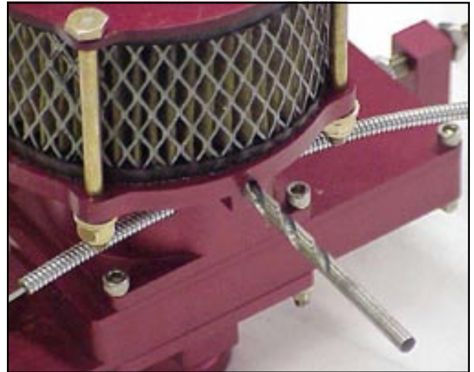
Figure 1.1 Twist, by hand, a 3/16" drill bit in one of the mounting holes to mark the bell of the AeroCarb.
